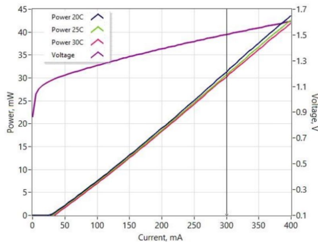
Light Current Voltage Characteristics
