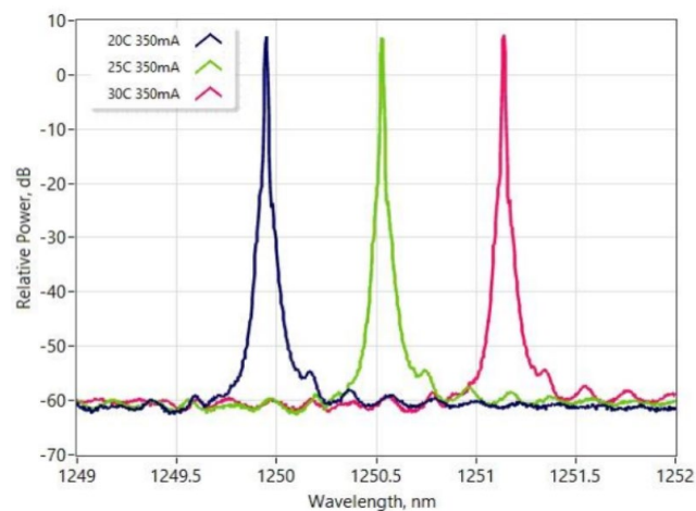
Optical Spectra vs Temperature (res. 10pm)
