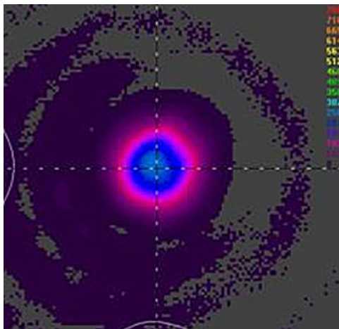
2-D Beam Profile at 762.0 mm (30.0 in)
