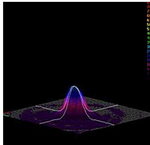
3-D Beam Profile at 762.0 mm (30.0 in)
